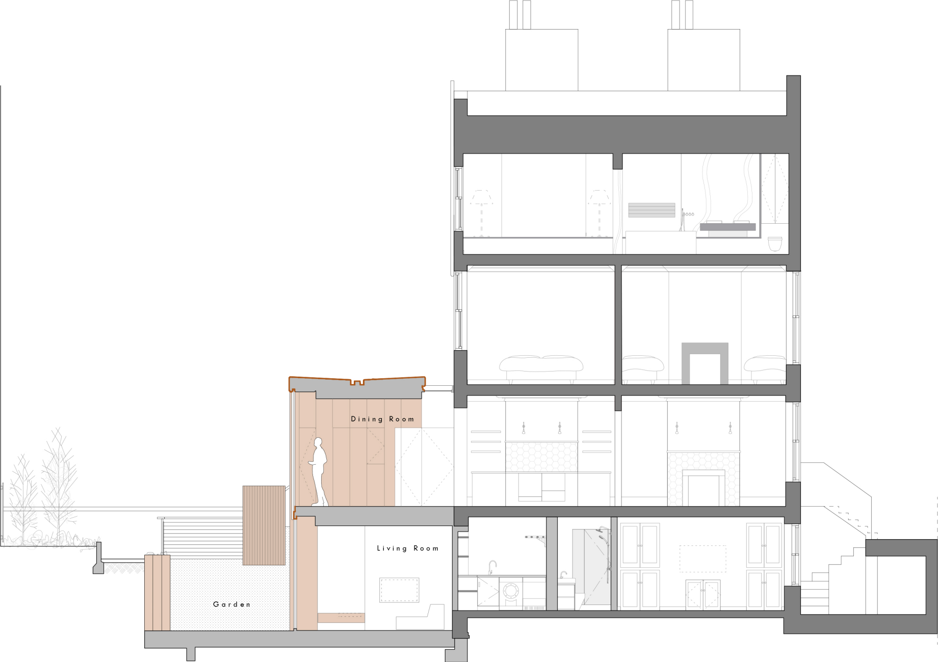
SECTION A-A Proposed
